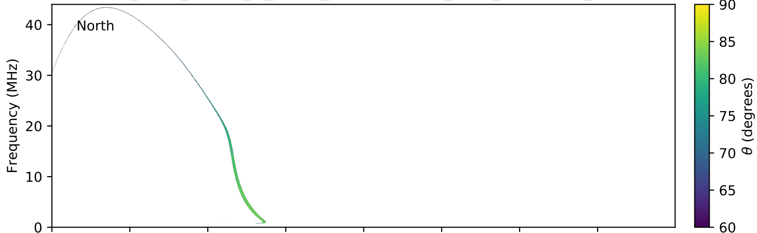
expres_earth_jupiter_io_jrm09_lossc-wid1deg_3kev_20050928_v01.cdf
