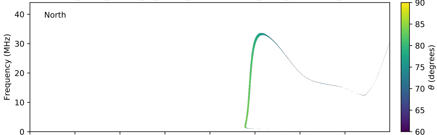
expres_earth_jupiter_io_jrm09_lossc-wid1deg_3kev_20050927_v01.cdf
