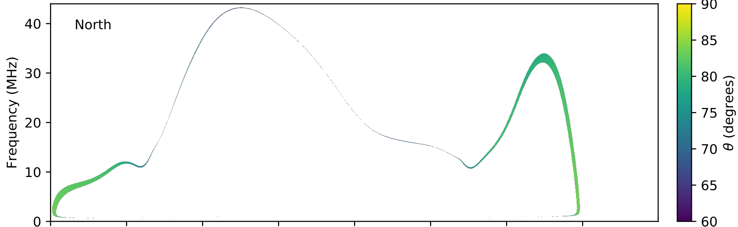
expres_earth_jupiter_io_jrm09_lossc-wid1deg_3kev_20050924_v01.cdf
