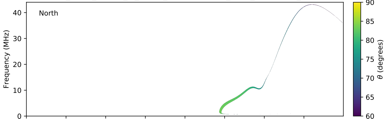
expres_earth_jupiter_io_jrm09_lossc-wid1deg_3kev_20050911_v01.cdf
