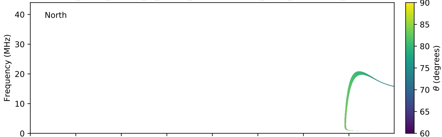
expres_earth_jupiter_io_jrm09_lossc-wid1deg_3kev_20050909_v01.cdf
