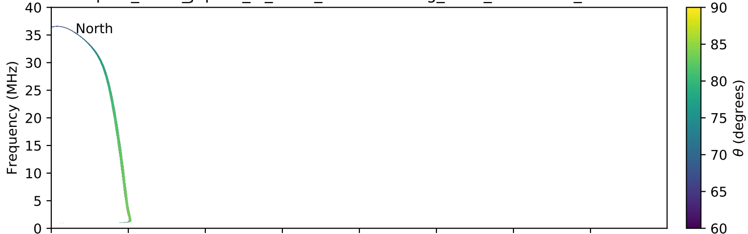
expres_earth_jupiter_io_isaac_lossc-wid1deg_3kev_20050930_v01.cdf
