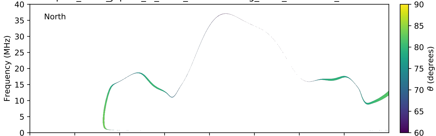
expres_earth_jupiter_io_isaac_lossc-wid1deg_3kev_20050922_v01.cdf
