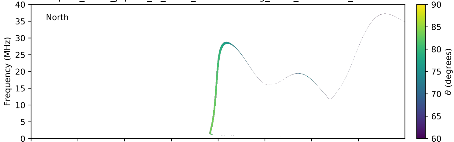
expres_earth_jupiter_io_isaac_lossc-wid1deg_3kev_20050920_v01.cdf
