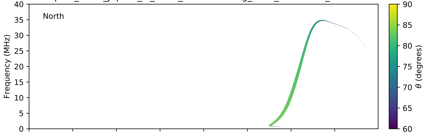
expres_earth_jupiter_io_isaac_lossc-wid1deg_3kev_20050918_v01.cdf
