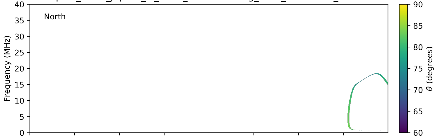
expres_earth_jupiter_io_isaac_lossc-wid1deg_3kev_20050916_v01.cdf
