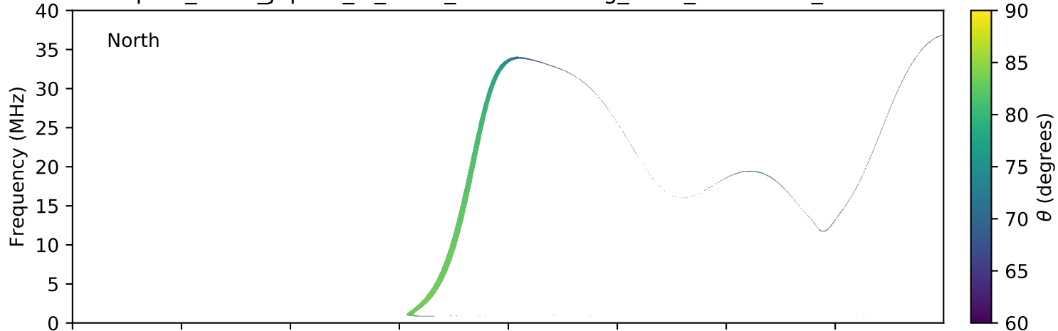
expres_earth_jupiter_io_isaac_lossc-wid1deg_3kev_20050913_v01.cdf
