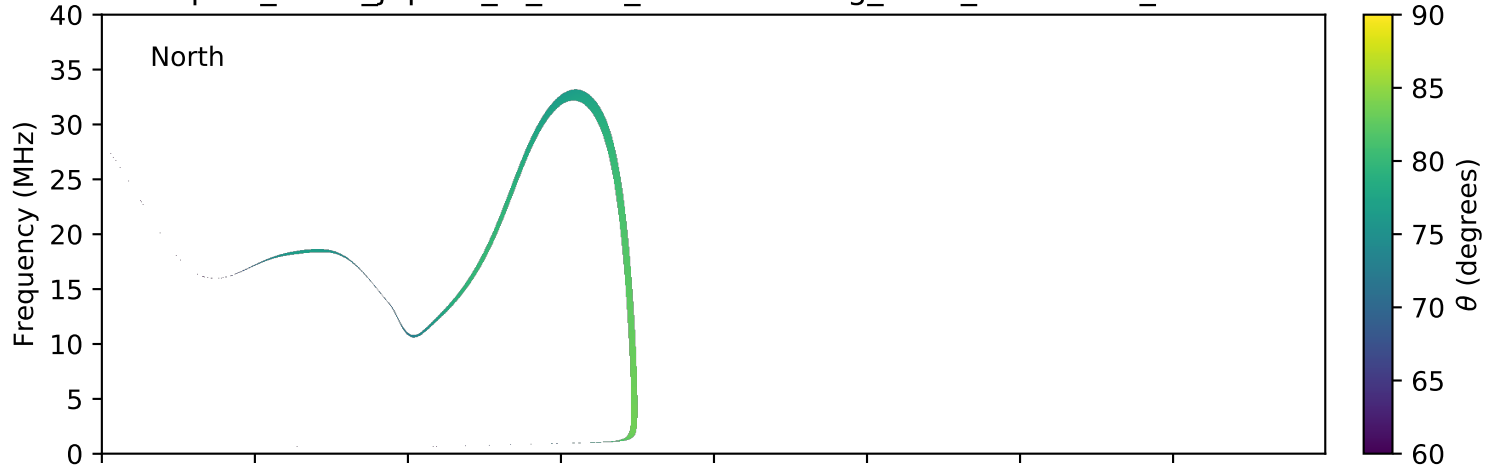
expres_earth_jupiter_io_isaac_lossc-wid1deg_3kev_20050912_v01.cdf
