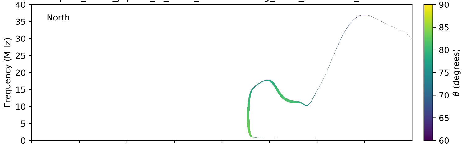
expres_earth_jupiter_io_isaac_lossc-wid1deg_3kev_20050911_v01.cdf
