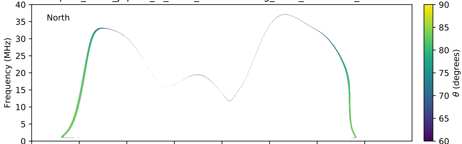
expres_earth_jupiter_io_isaac_lossc-wid1deg_3kev_20050908_v01.cdf
