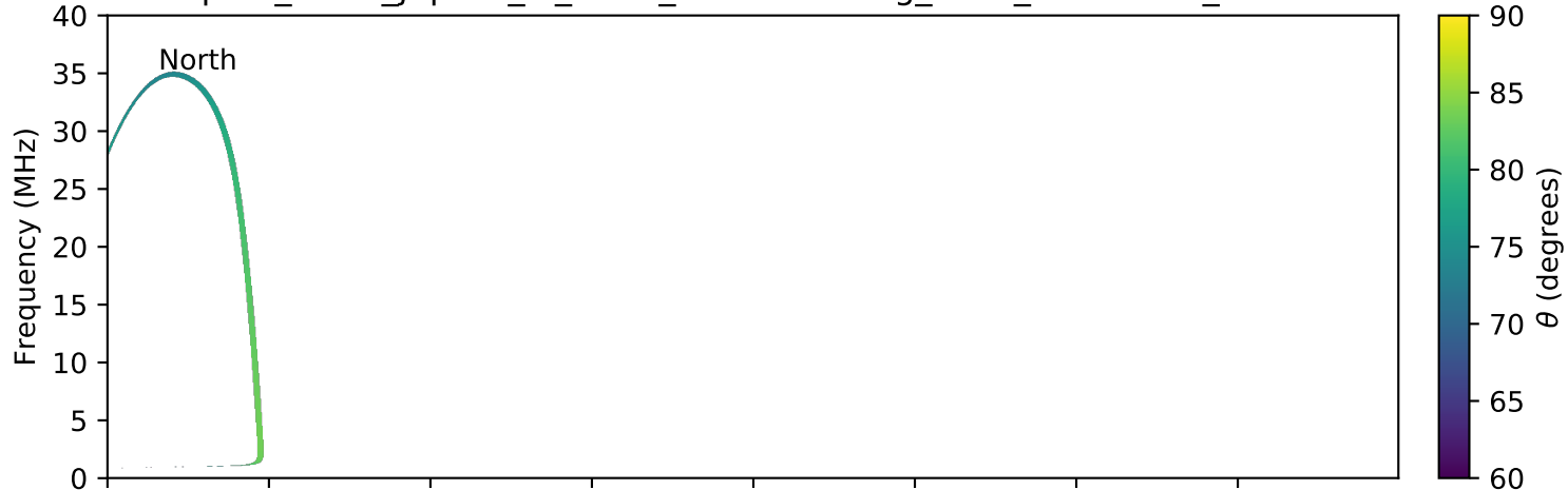
expres_earth_jupiter_io_isaac_lossc-wid1deg_3kev_20050907_v01.cdf
