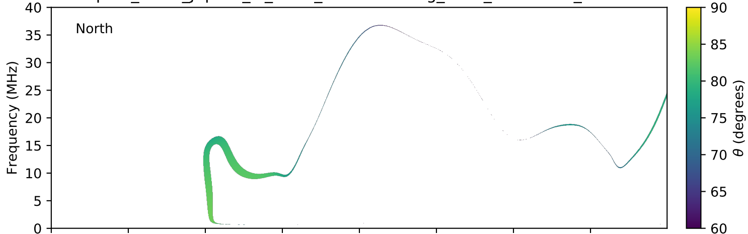
expres_earth_jupiter_io_isaac_lossc-wid1deg_3kev_20050906_v01.cdf
