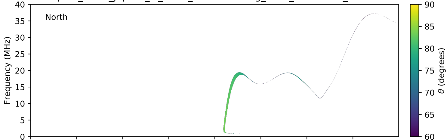
expres_earth_jupiter_io_isaac_lossc-wid1deg_3kev_20050904_v01.cdf
