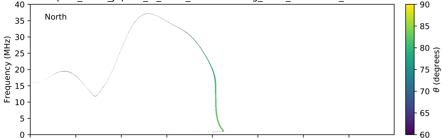
expres_earth_jupiter_io_isaac_lossc-wid1deg_3kev_20050903_v01.cdf
