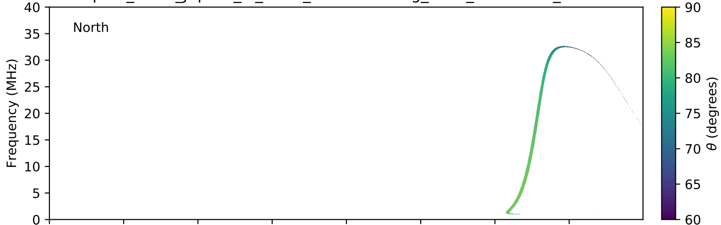
expres_earth_jupiter_io_isaac_lossc-wid1deg_3kev_20050902_v01.cdf
