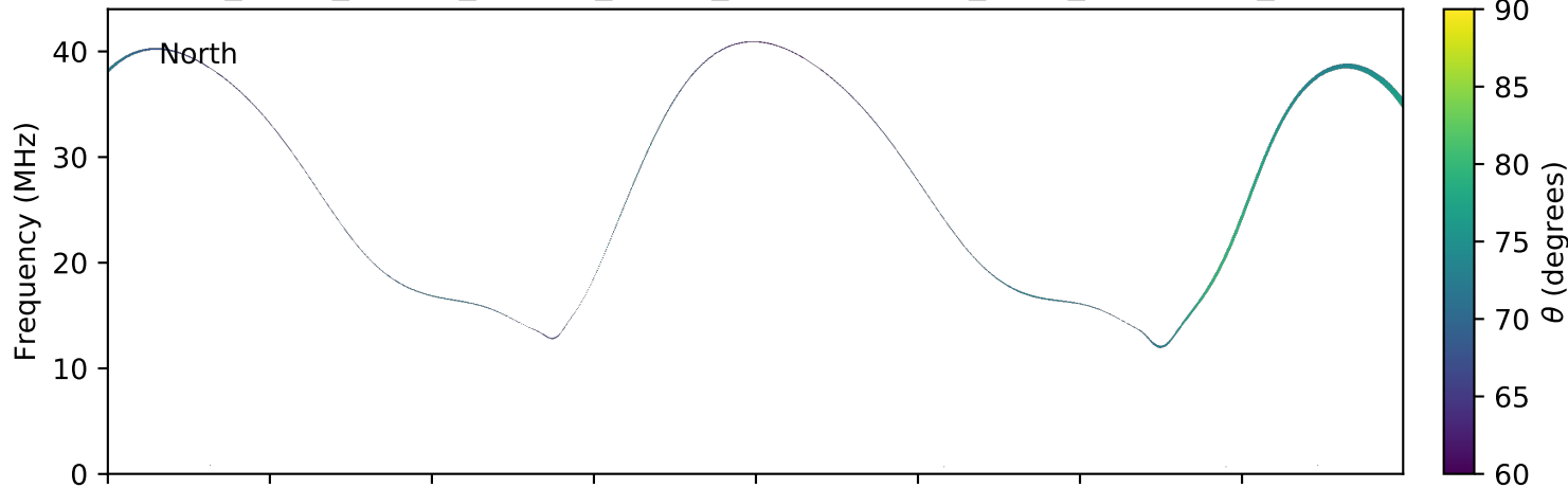
expres_earth_jupiter_europa_jrm09_lossc-wid1deg_3kev_20050928_v01.cdf
