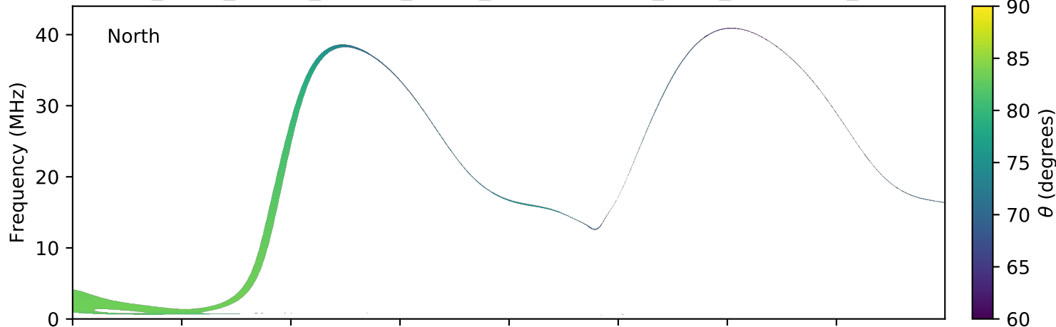
expres_earth_jupiter_europa_jrm09_lossc-wid1deg_3kev_20050924_v01.cdf
