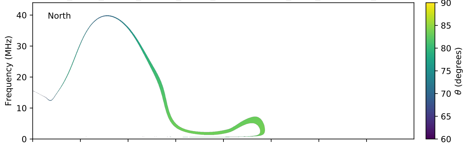
expres_earth_jupiter_europa_jrm09_lossc-wid1deg_3kev_20050918_v01.cdf
