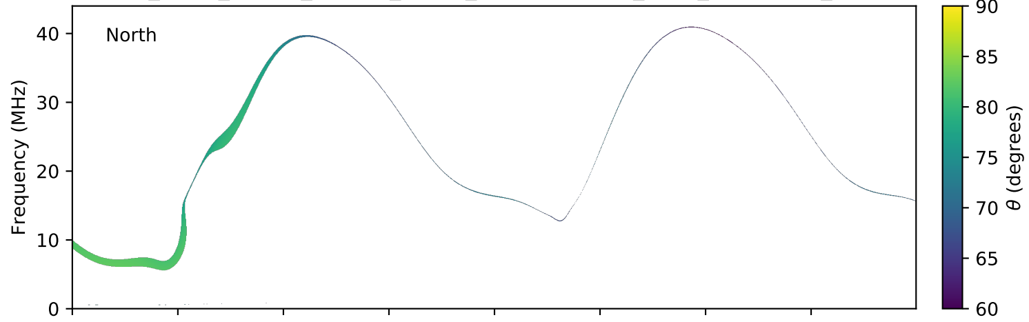
expres_earth_jupiter_europa_jrm09_lossc-wid1deg_3kev_20050917_v01.cdf
