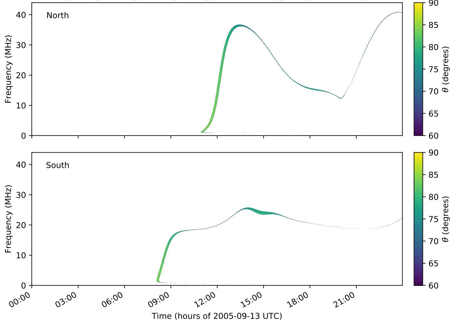
expres_earth_jupiter_europa_jrm09_lossc-wid1deg_3kev_20050913_v01.cdf
