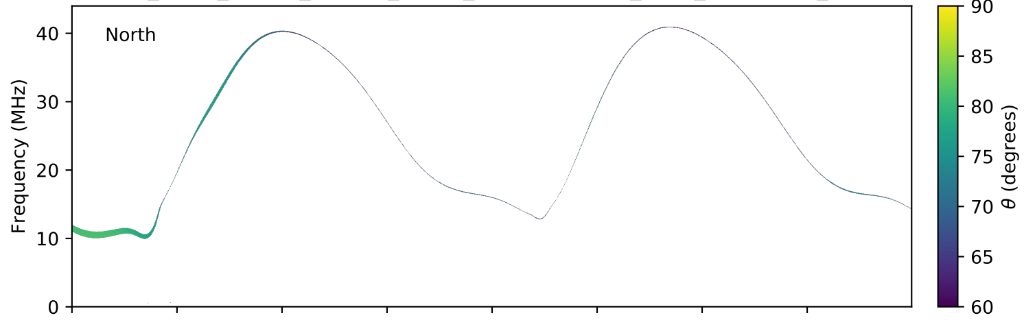
expres_earth_jupiter_europa_jrm09_lossc-wid1deg_3kev_20050910_v01.cdf
