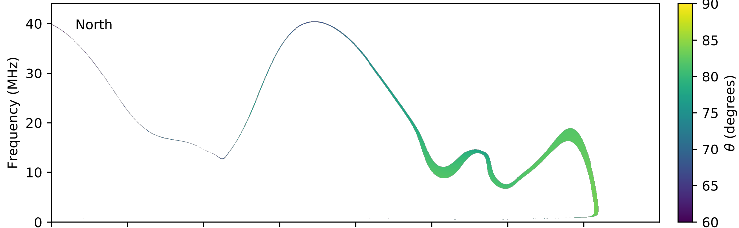
expres_earth_jupiter_europa_jrm09_lossc-wid1deg_3kev_20050907_v01.cdf
