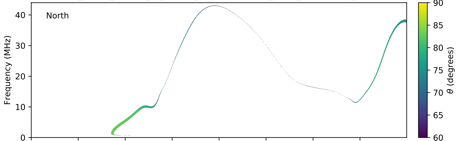
expres_earth_jupiter_io_jrm09_lossc-wid1deg_3kev_20050830_v01.cdf
