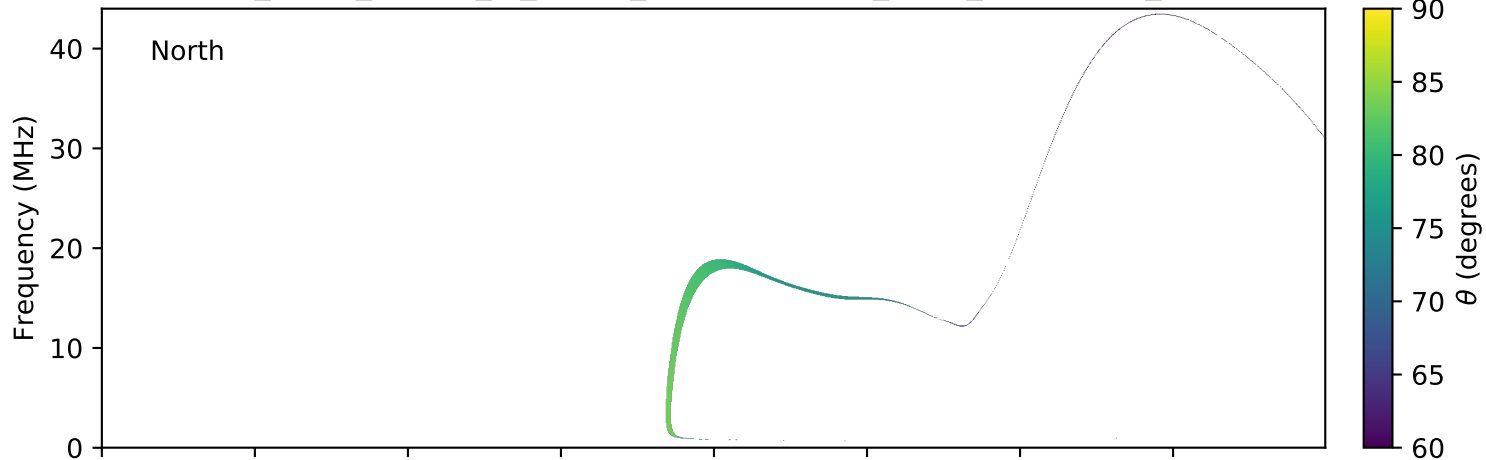
expres_earth_jupiter_io_jrm09_lossc-wid1deg_3kev_20050828_v01.cdf
