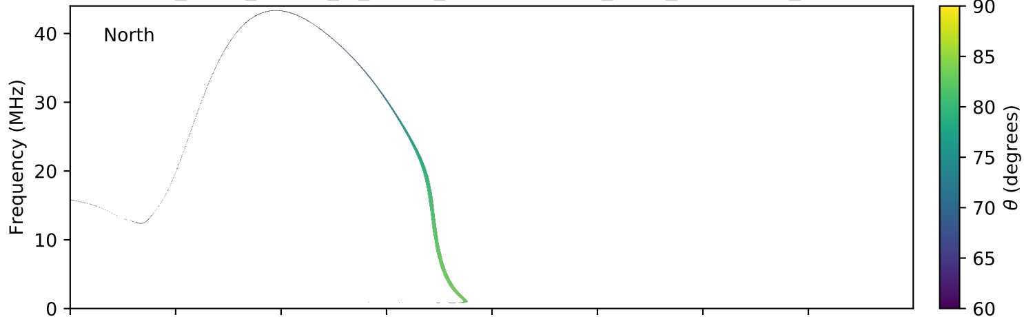
expres_earth_jupiter_io_jrm09_lossc-wid1deg_3kev_20050827_v01.cdf
