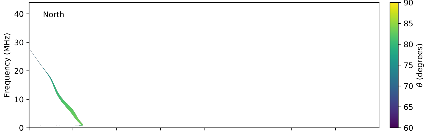
expres_earth_jupiter_io_jrm09_lossc-wid1deg_3kev_20050822_v01.cdf
