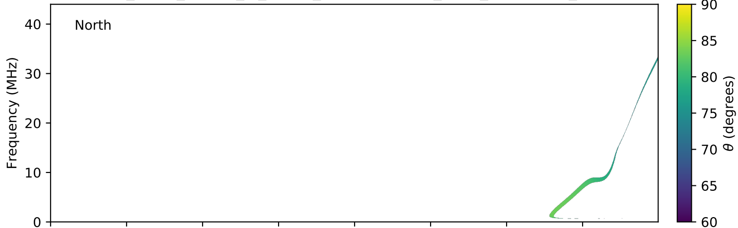
expres_earth_jupiter_io_jrm09_lossc-wid1deg_3kev_20050817_v01.cdf
