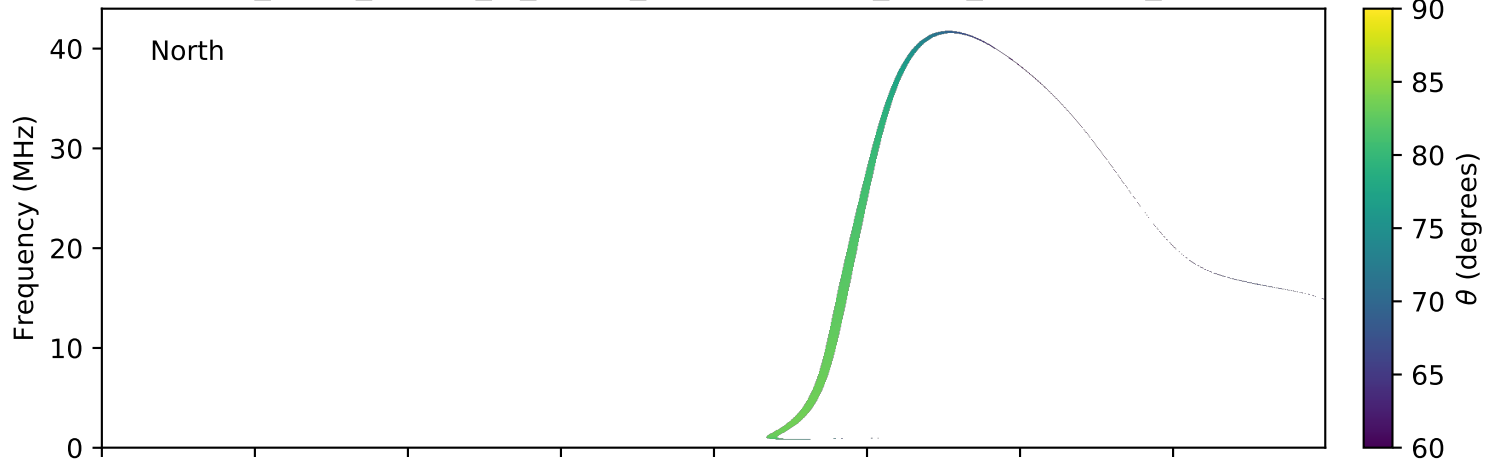
expres_earth_jupiter_io_jrm09_lossc-wid1deg_3kev_20050812_v01.cdf
