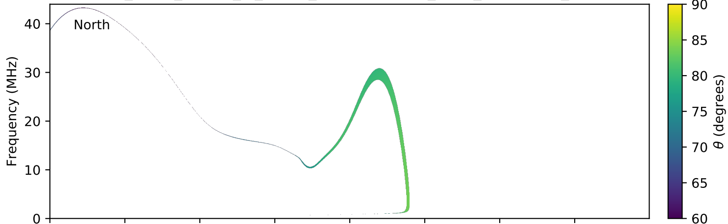
expres_earth_jupiter_io_jrm09_lossc-wid1deg_3kev_20050811_v01.cdf
