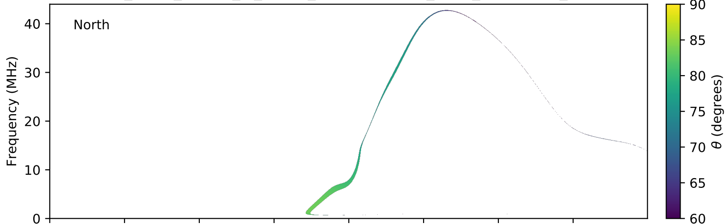
expres_earth_jupiter_io_jrm09_lossc-wid1deg_3kev_20050805_v01.cdf
