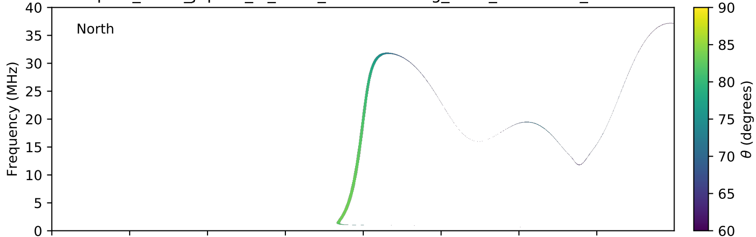
expres_earth_jupiter_io_isaac_lossc-wid1deg_3kev_20050828_v01.cdf
