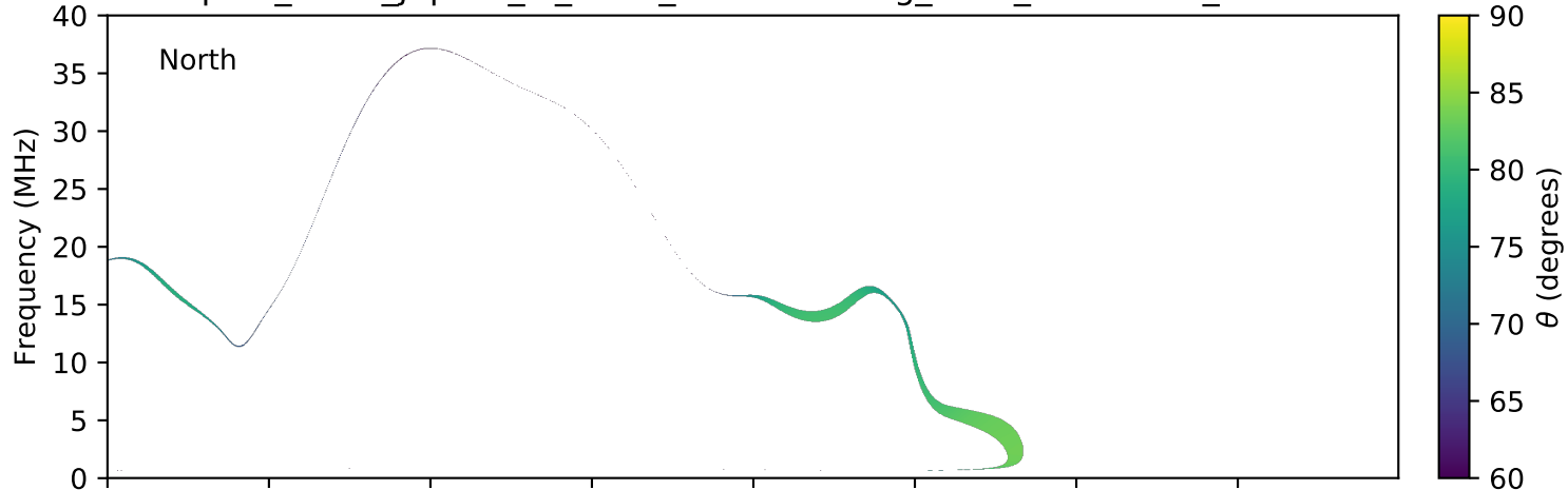
expres_earth_jupiter_io_isaac_lossc-wid1deg_3kev_20050825_v01.cdf
