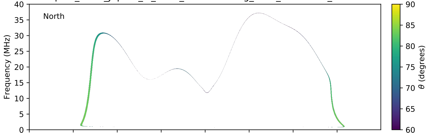
expres_earth_jupiter_io_isaac_lossc-wid1deg_3kev_20050823_v01.cdf
