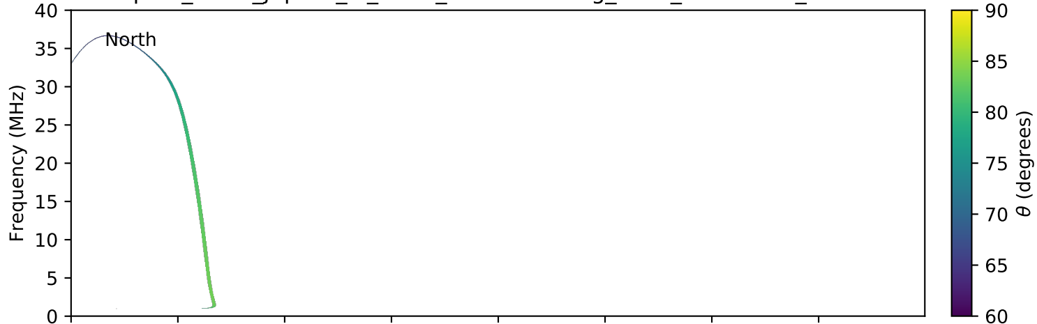
expres_earth_jupiter_io_isaac_lossc-wid1deg_3kev_20050822_v01.cdf
