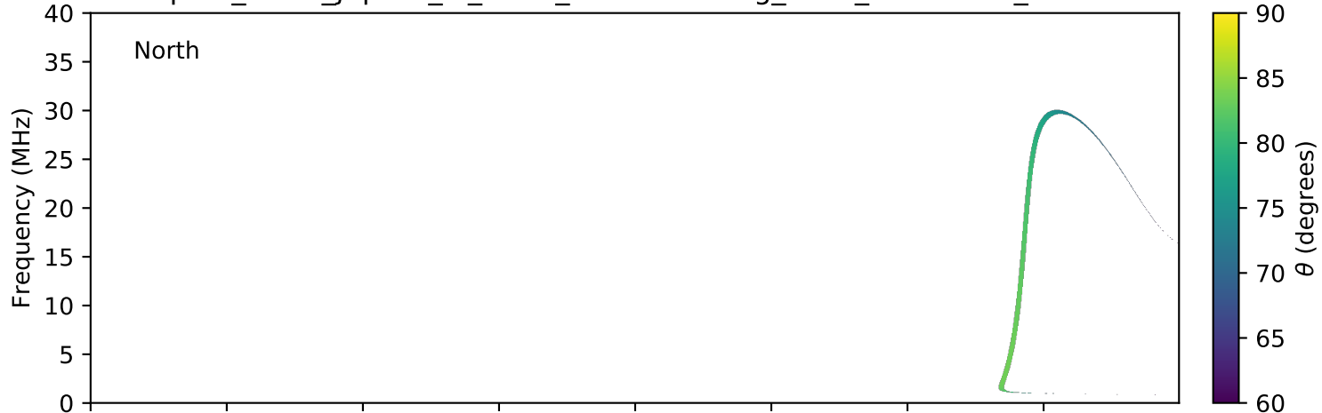
expres_earth_jupiter_io_isaac_lossc-wid1deg_3kev_20050817_v01.cdf
