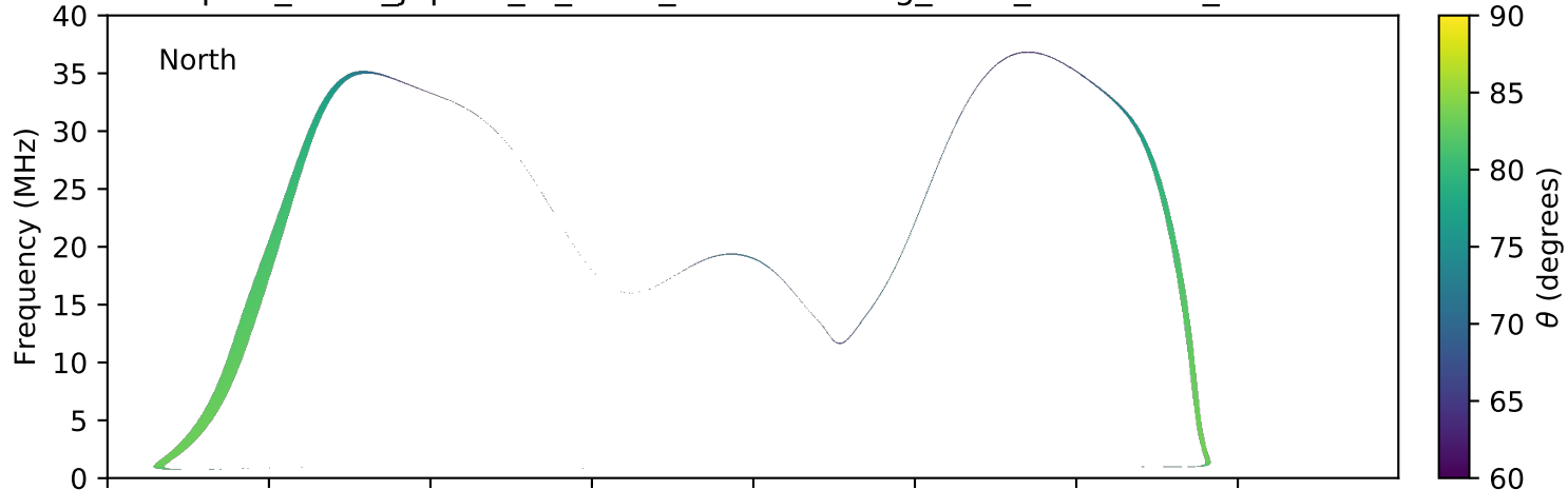
expres_earth_jupiter_io_isaac_lossc-wid1deg_3kev_20050816_v01.cdf
