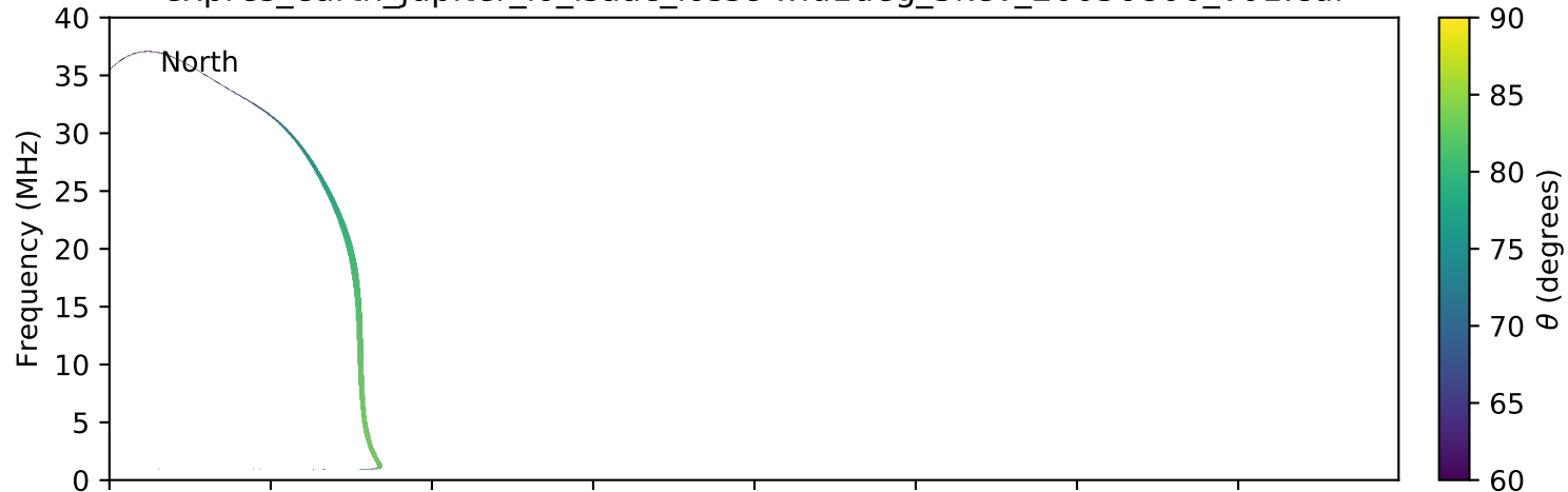
expres_earth_jupiter_io_isaac_lossc-wid1deg_3kev_20050806_v01.cdf
