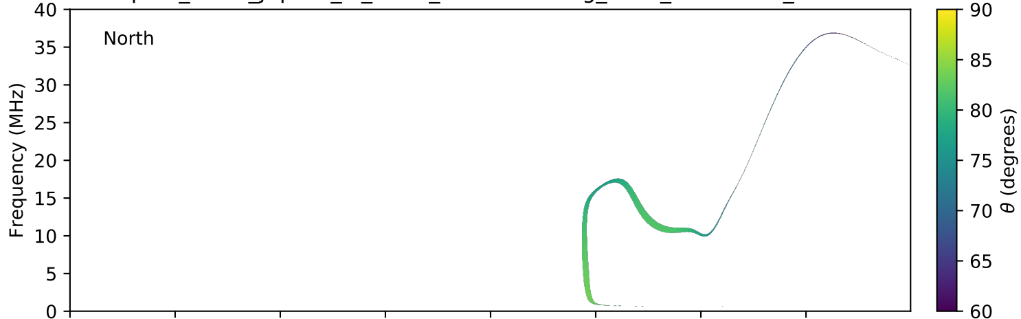
expres_earth_jupiter_io_isaac_lossc-wid1deg_3kev_20050803_v01.cdf
