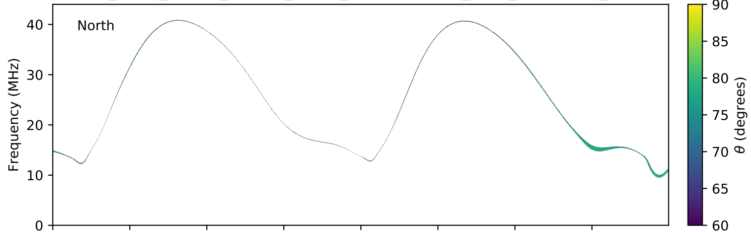
expres_earth_jupiter_europa_jrm09_lossc-wid1deg_3kev_20050827_v01.cdf
