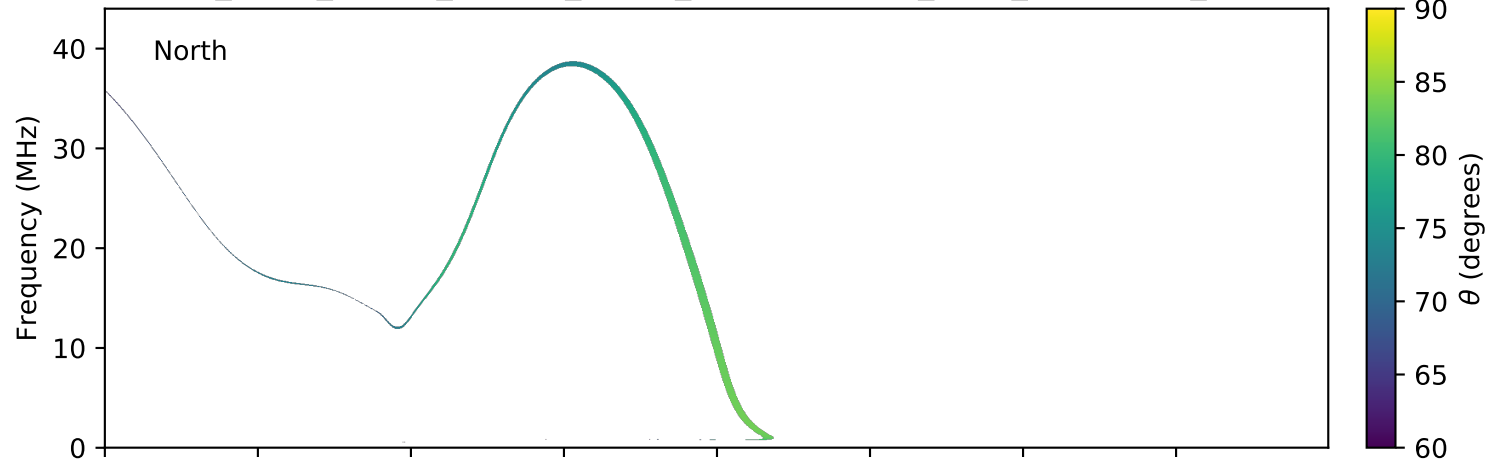
expres_earth_jupiter_europa_jrm09_lossc-wid1deg_3kev_20050824_v01.cdf
