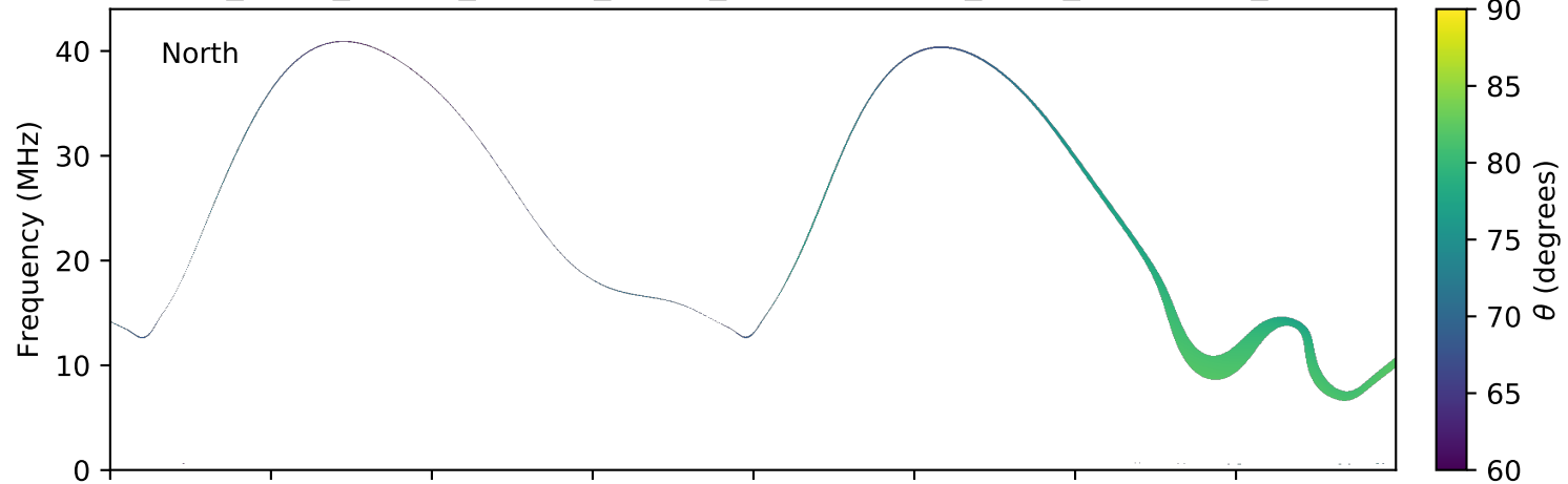
expres_earth_jupiter_europa_jrm09_lossc-wid1deg_3kev_20050820_v01.cdf
