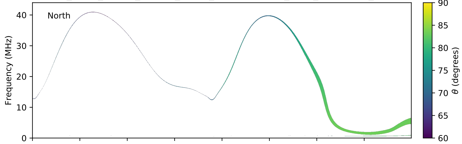
expres_earth_jupiter_europa_jrm09_lossc-wid1deg_3kev_20050813_v01.cdf
