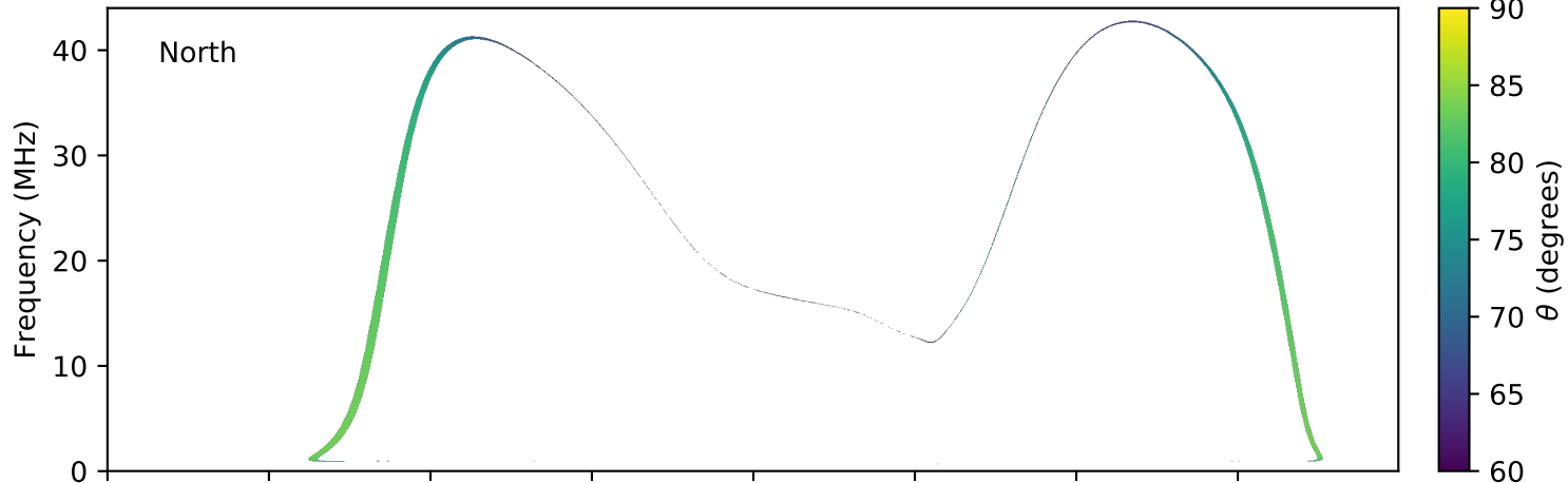
expres_earth_jupiter_io_jrm09_lossc-wid1deg_3kev_20050731_v01.cdf
