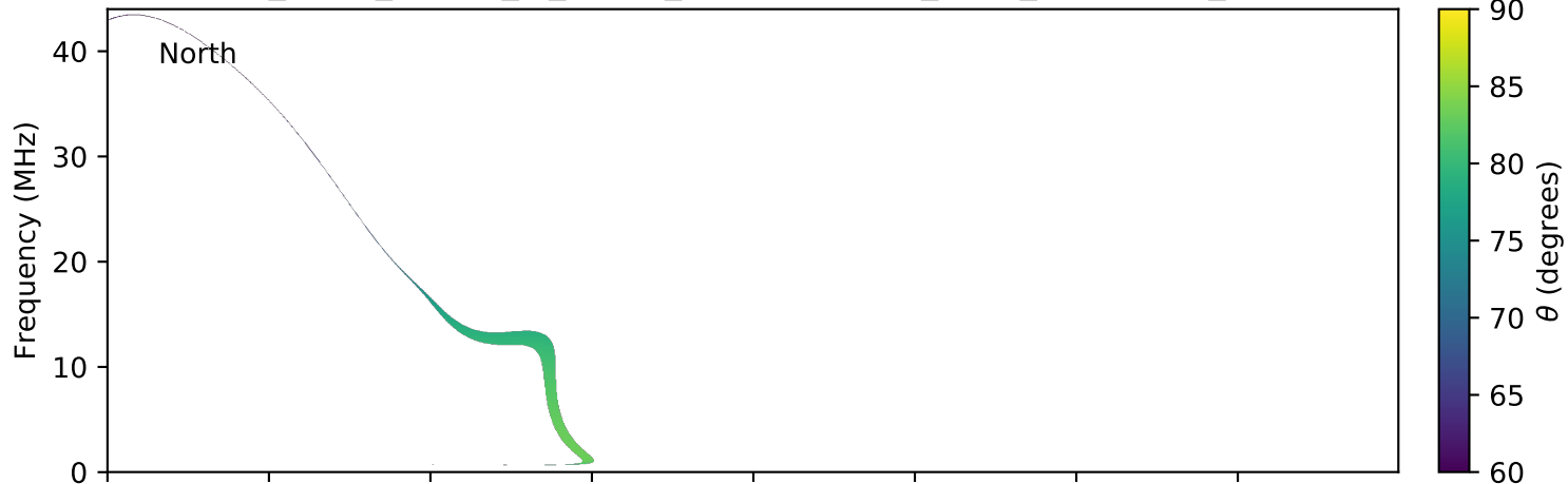
expres_earth_jupiter_io_jrm09_lossc-wid1deg_3kev_20050728_v01.cdf
