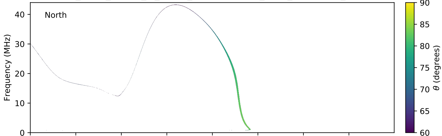
expres_earth_jupiter_io_jrm09_lossc-wid1deg_3kev_20050726_v01.cdf
