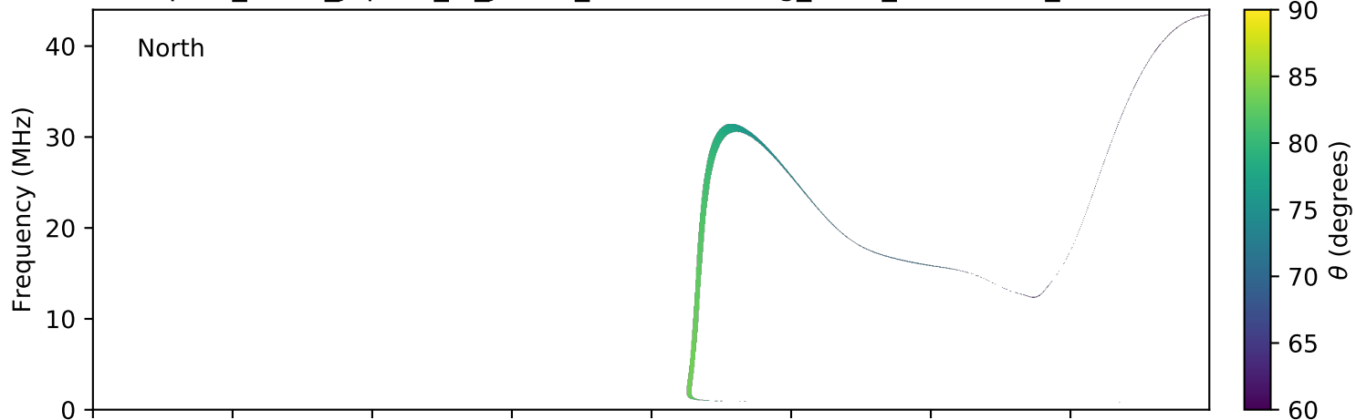
expres_earth_jupiter_io_jrm09_lossc-wid1deg_3kev_20050720_v01.cdf
